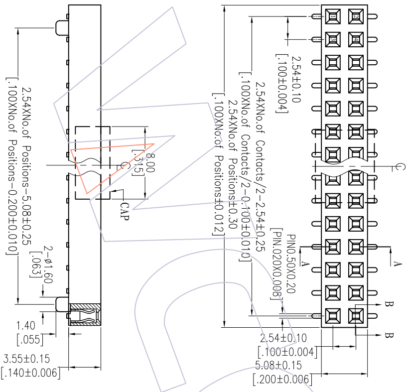
SECTION B-B
